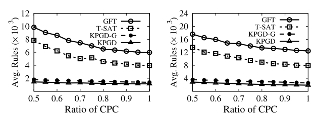
Fig. 15. Avg. Rules vs. Ratio of CPC. Left plot: Topology (a); right plot: Topology (b).
